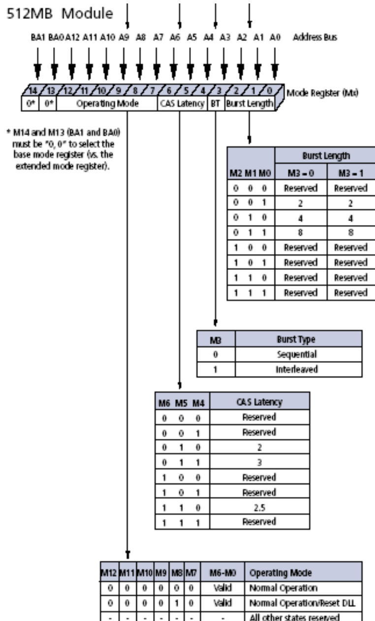
Figure 4: Mode Register Definition Diagram
