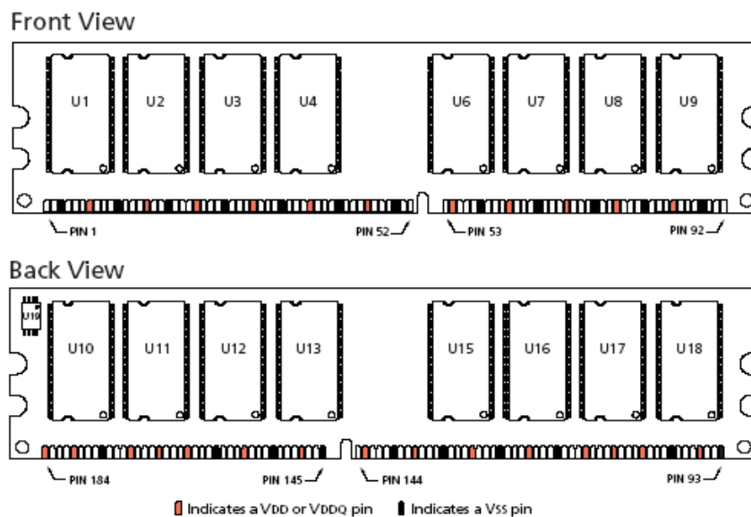
Figure 2: Pin Locations
