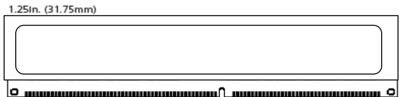
Figure 1: 184-Pin DIMM
